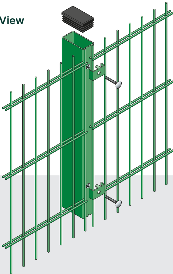
Exploded view of post and fixing detail for Dulok-Lite double wire panel system
